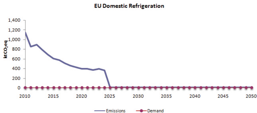
Figure 2.2 HFC demand and (end-of-life) emissions in the EU under the current F-Gas Regulation assuming full implementation for domestic refrigeration 2010-2050. In Europe, household refrigerators and freezers use hydrocarbons as refrigerants. Demand for domestic manufacturing will be of negligible size from 2010 onwards. Emissions from disposal will likewise decrease to marginal amounts from 2025. 61
