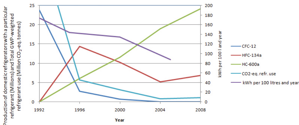
Figure 2.1 Annual European production of domestic refrigerators and freezers in million units and the CO 2 -equivalent weighted refrigerant consumption as well as specific energy consumption 54 of combined refrigerator-freezers. 55
